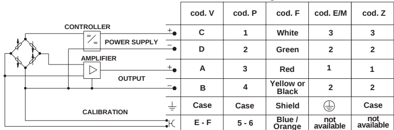
VOLTAGE AMPLIFIED OUTPUT - mod. B/C/M/N/P/Q/R
