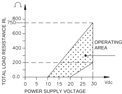
LOAD DIAGRAM (Current output)
