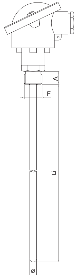
TC6M D with welded fitting under the head
